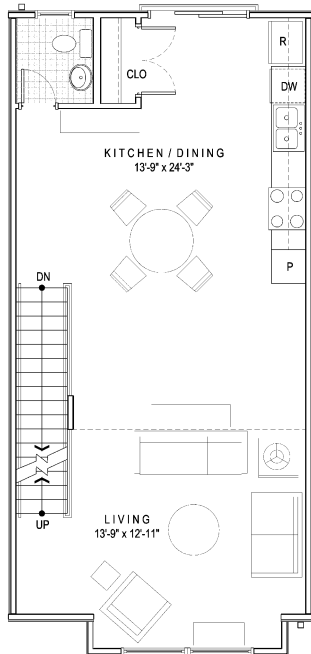
2nd Level Plan
